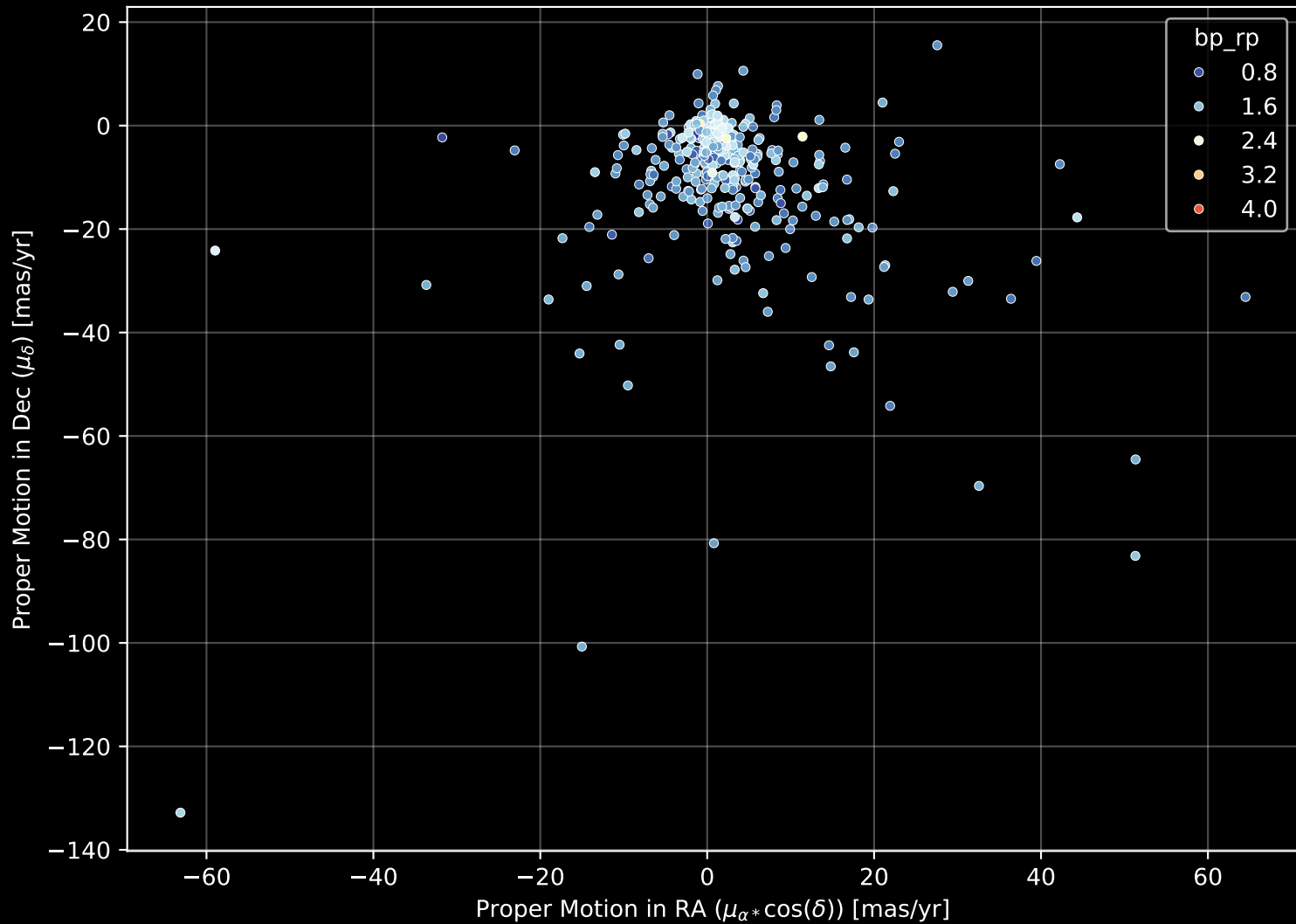
GALAH DR4 Field: [6775] Proper Motion Diagram (n= 432)
