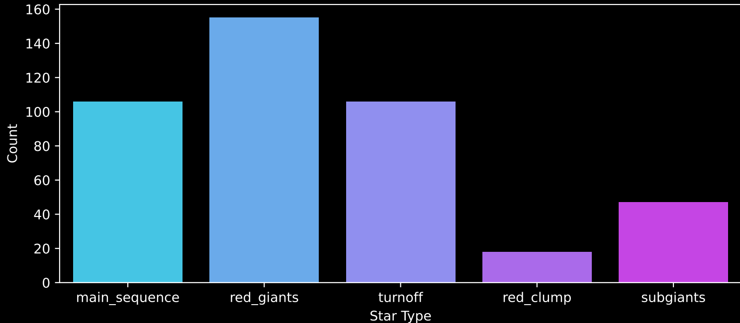
GALAH DR4 Field: [6775] Count plot of Star Type
