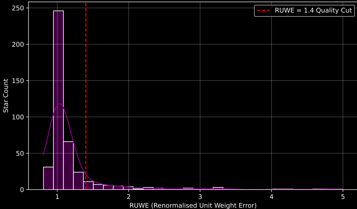
GALAH DR4 Field [6775] RUWE Distribution (n= 418)
